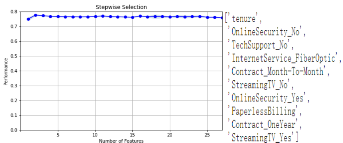
Figure 3. One-hot Encoded Variables Selected by Wrapper.
