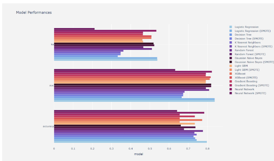
Figure 4. Model Performances for Target Encoded Data.
